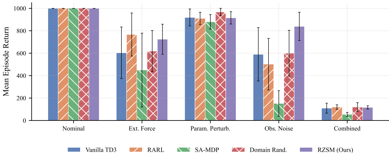
InvertedPendulum-v5: Performance Under Disturbance Scenarios (5 seeds)
