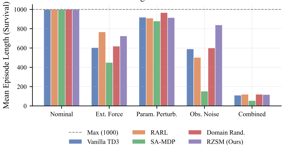
InvertedPendulum-v5: Agent Survival Under Disturbances
