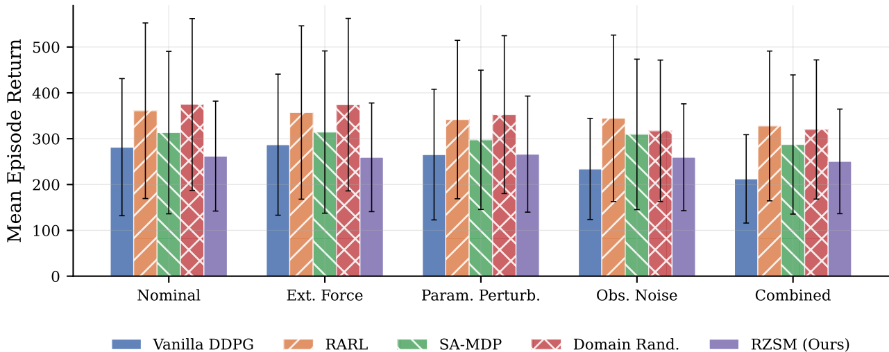
Hopper-v5: Performance Under Disturbance Scenarios (5 seeds)
