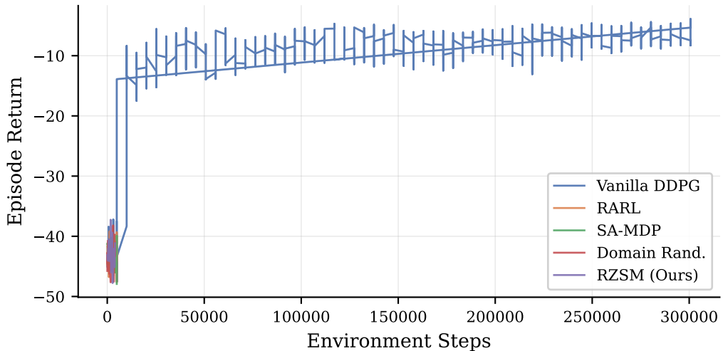
Training Curves — Reacher-v5
