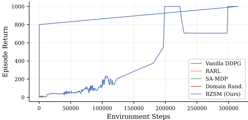
Training Curves — InvertedPendulum-v5
