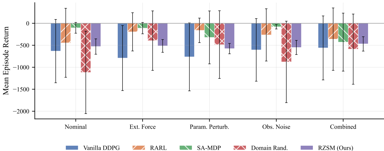
Ant-v5: Performance Under Disturbance Scenarios
