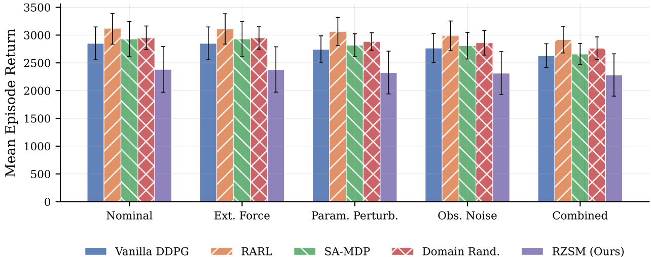
HalfCheetah-v5: Performance Under Disturbance Scenarios (5 seeds)
