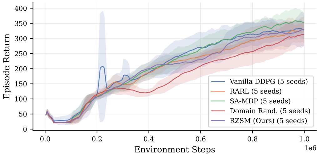
Training Curves — InvertedDoublePendulum-v5 (mean \pm std, 5 seeds)
