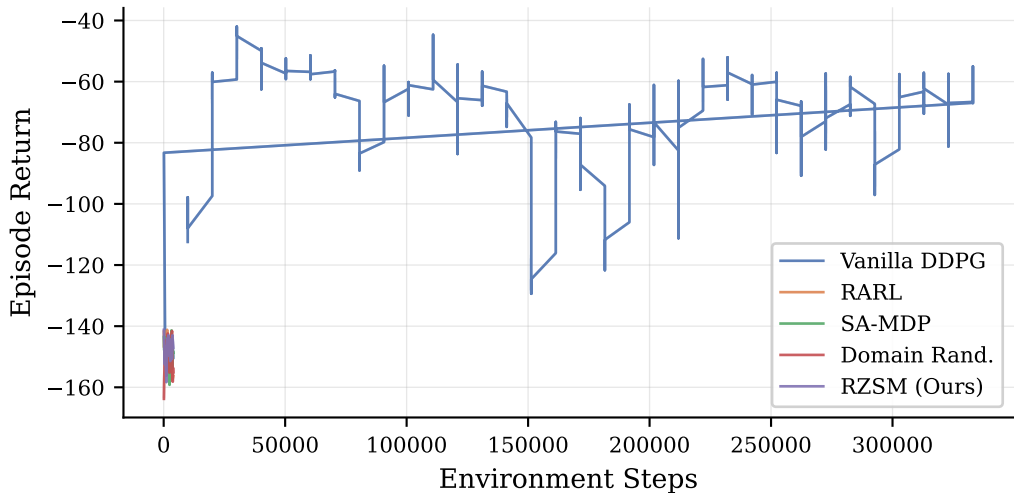
Training Curves — Pusher-v5
