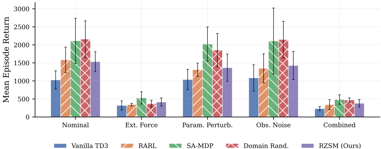
Ant-v5: Performance Under Disturbance Scenarios (5 seeds)
