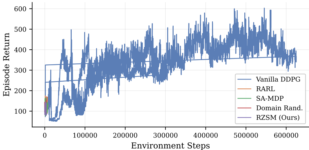
Training Curves — Humanoid-v5
