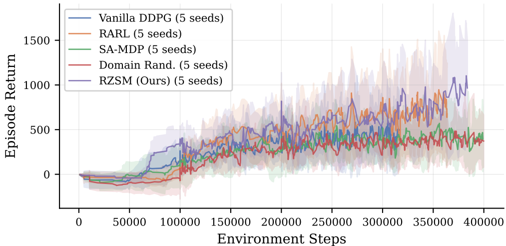
Training Curves — Ant-v5 (mean \pm std, 5 seeds)
