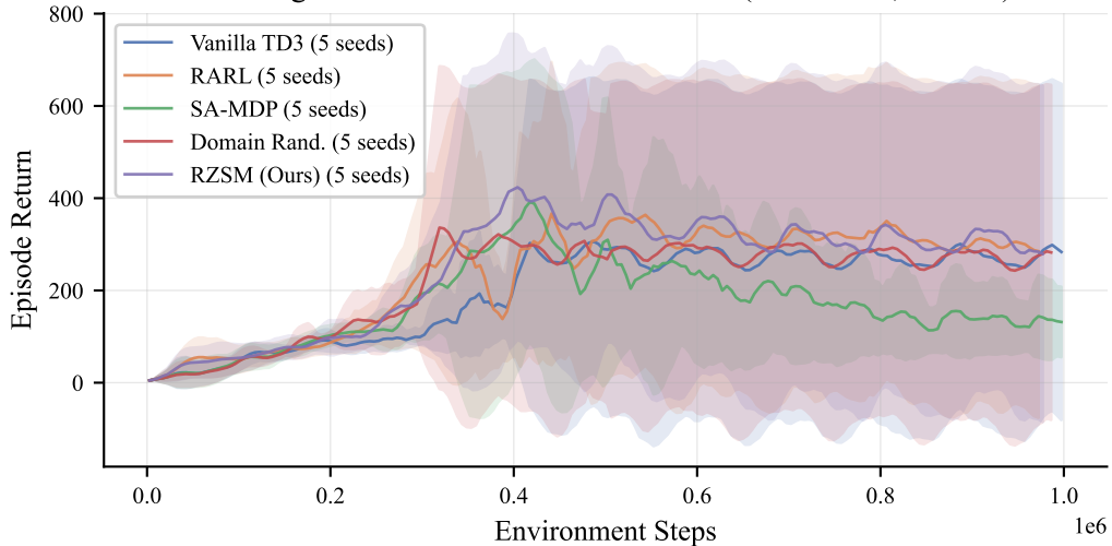
Training Curves — InvertedPendulum-v5 (mean \pm std, 5 seeds)
