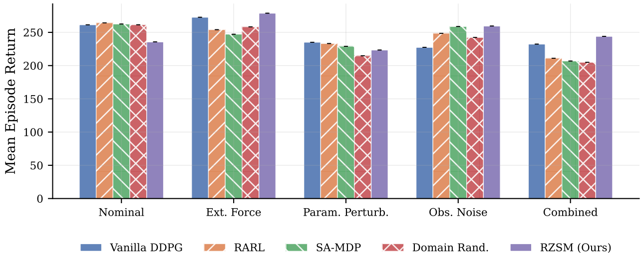
Humanoid-v5: Performance Under Disturbance Scenarios
