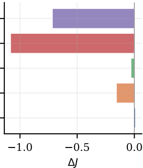
Obs. Noise
