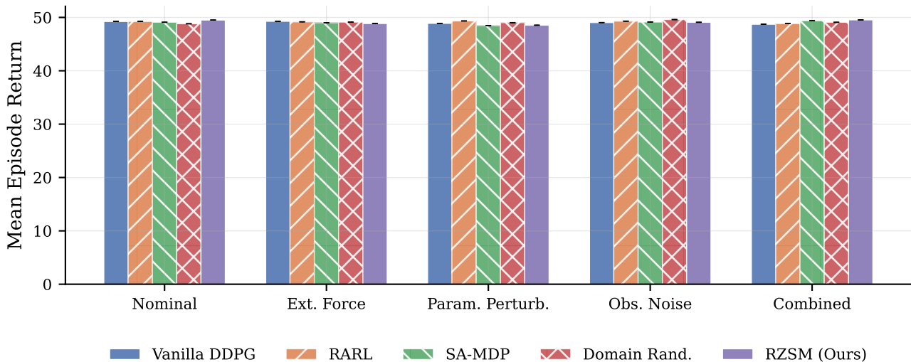
Walker2d-v5: Performance Under Disturbance Scenarios
