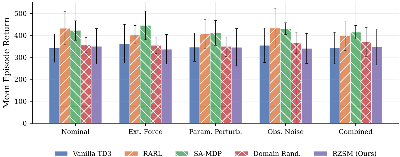
Humanoid-v5: Performance Under Disturbance Scenarios (5 seeds)
