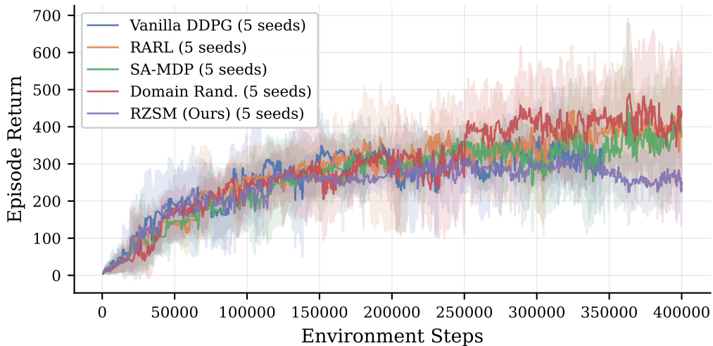
Training Curves — Hopper-v5 (mean \pm std, 5 seeds)
