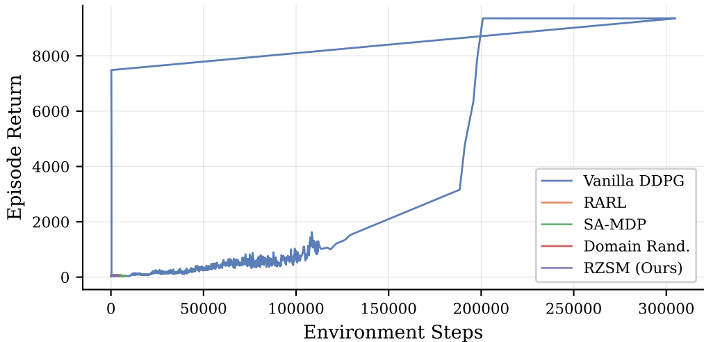
Training Curves — InvertedDoublePendulum-v5
