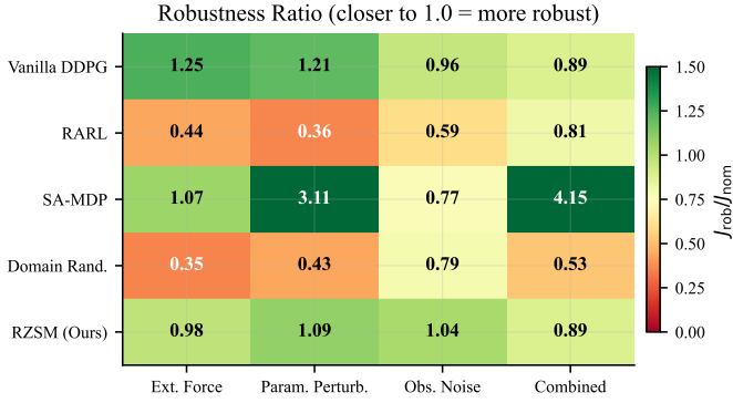
Fig. 2: Robustness ratio heatmap. Green indicates ratios near 1.0 (minimal degradation), red indicates large deviations. RZSM (bottom row) shows the most uniform green pattern across all disturbance types.
