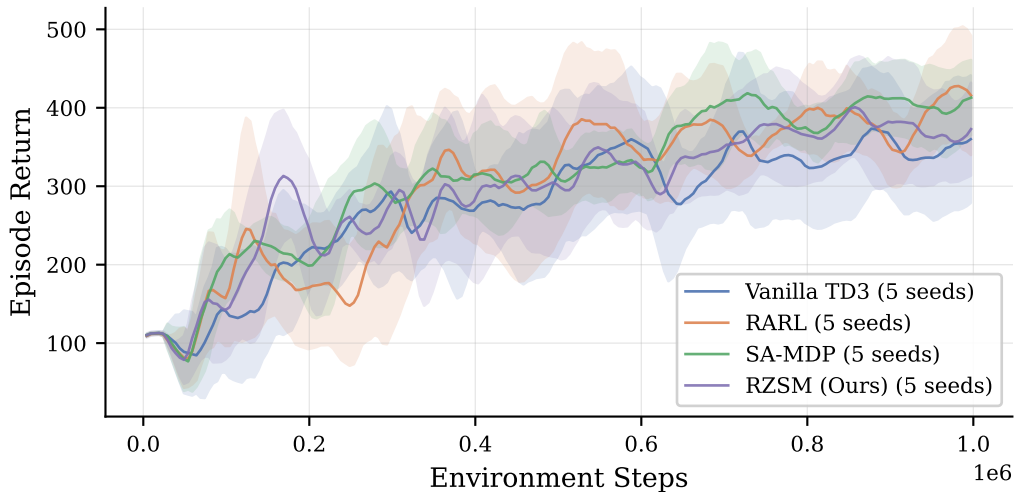
Training Curves — Humanoid-v5 (mean \pm std, 5 seeds)
