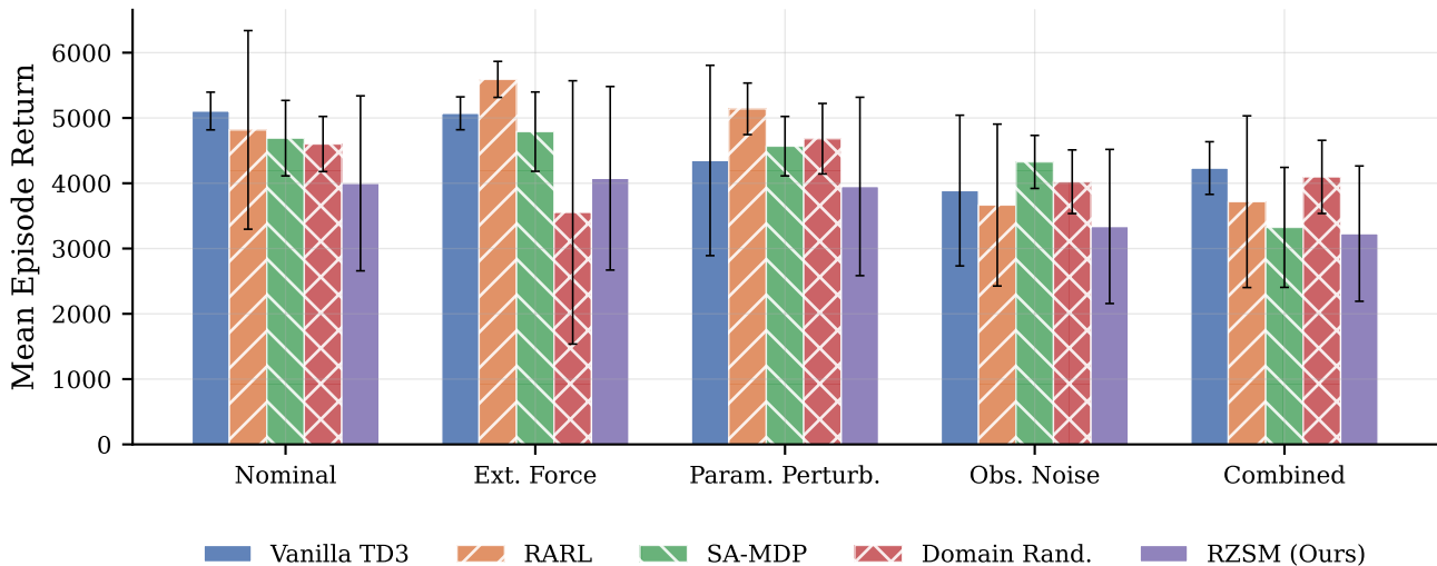
HalfCheetah-v5: Performance Under Disturbance Scenarios (5 seeds)
