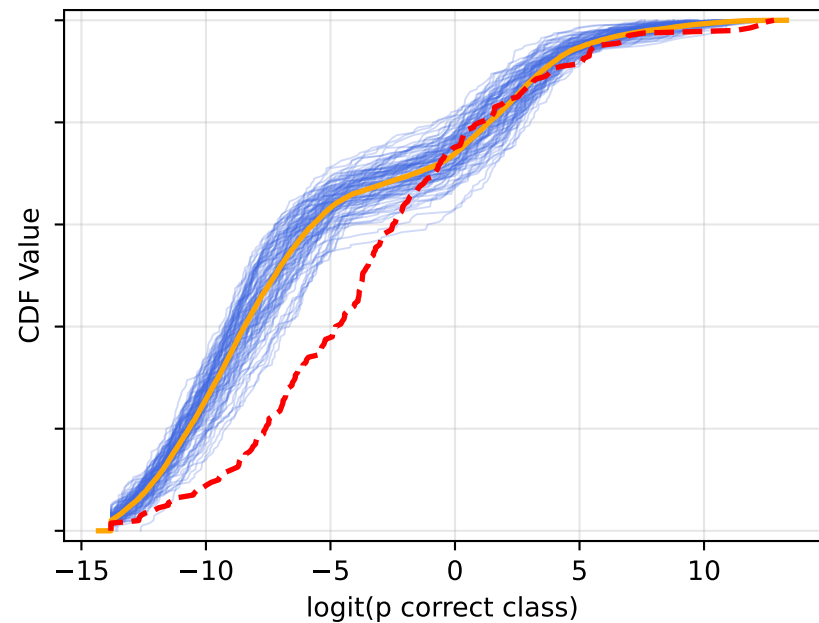
Deepseek v4 Pro Split = 200 (acc=27.0%) (K=100)
