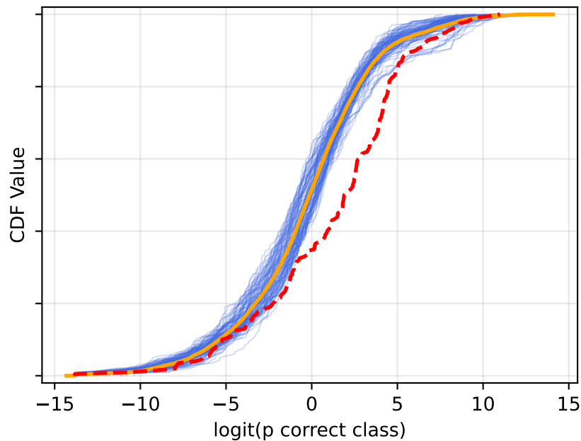
GPT 4o Split = 200 (acc=65.5%) (K=100)
