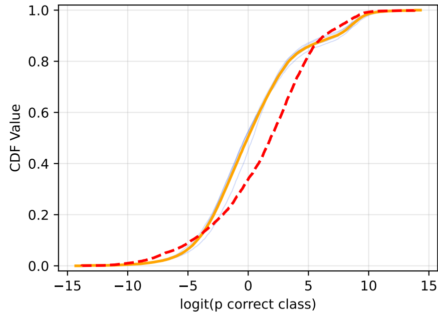
GPT 4o Split = All (acc=68.4%) (K=5)
