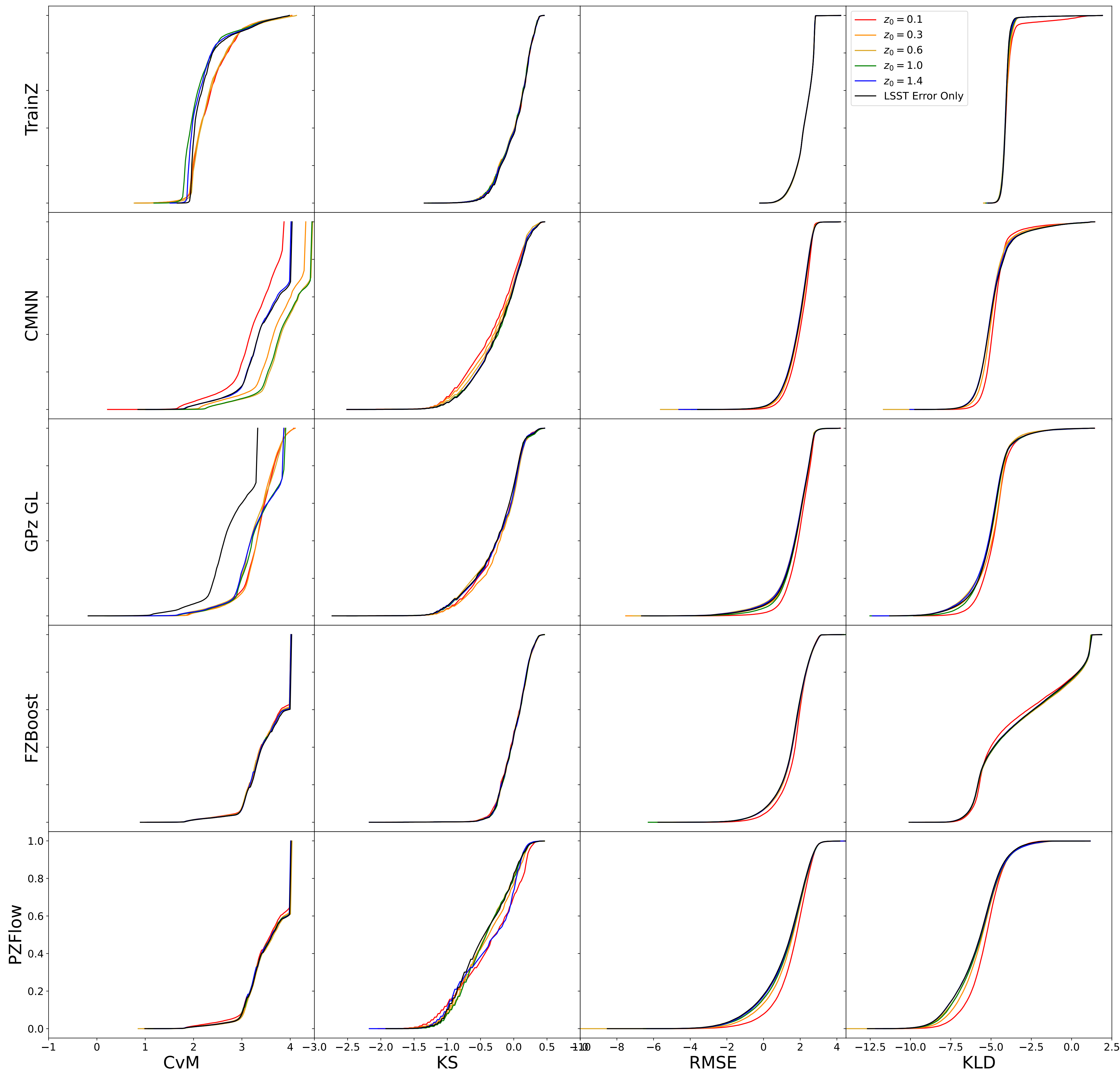
Summary Statistic Quantile Plots for Inverse Redshift Incompleteness Degradation
