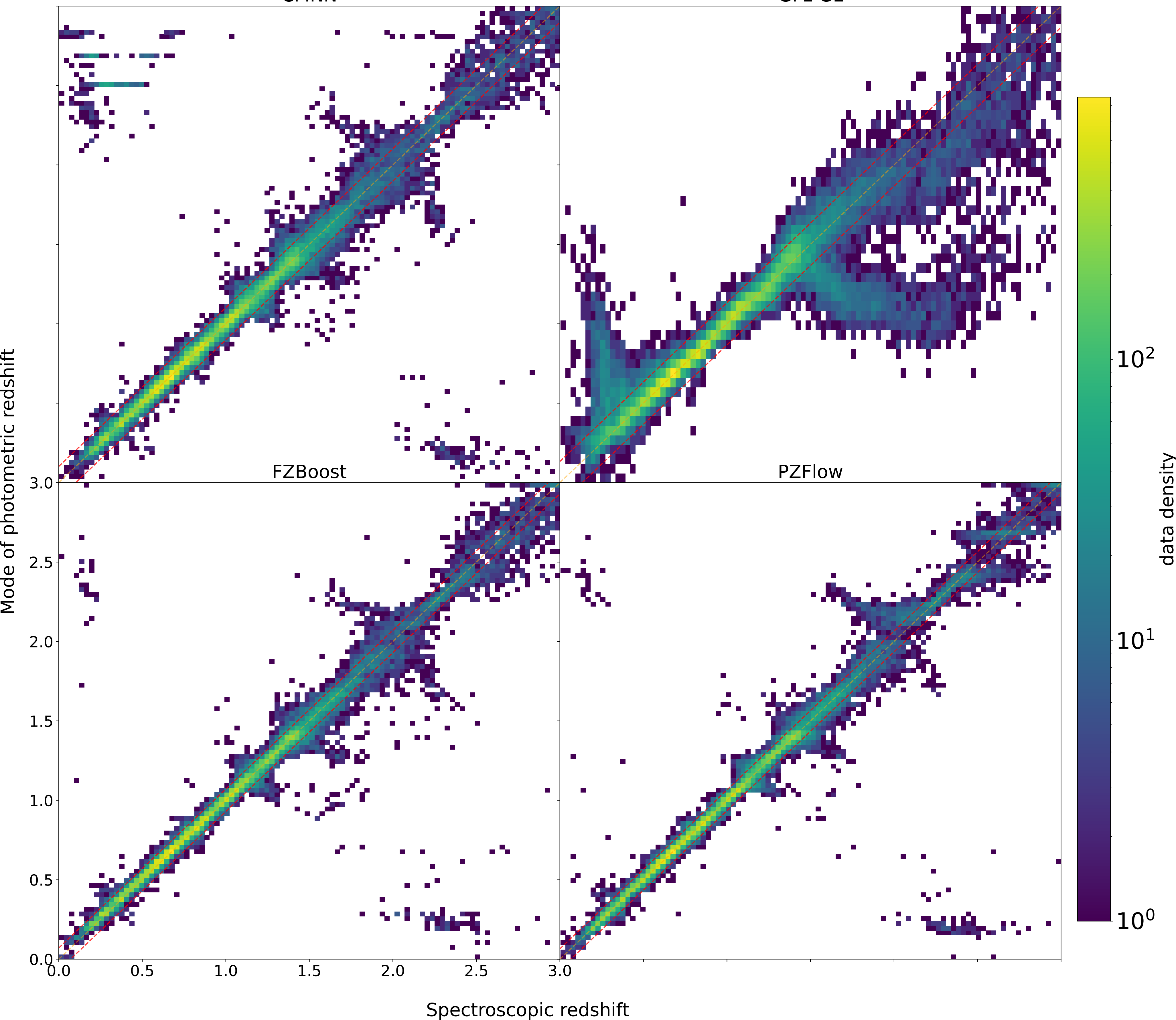
Mode point estimates for LSST error model only training set degradation
