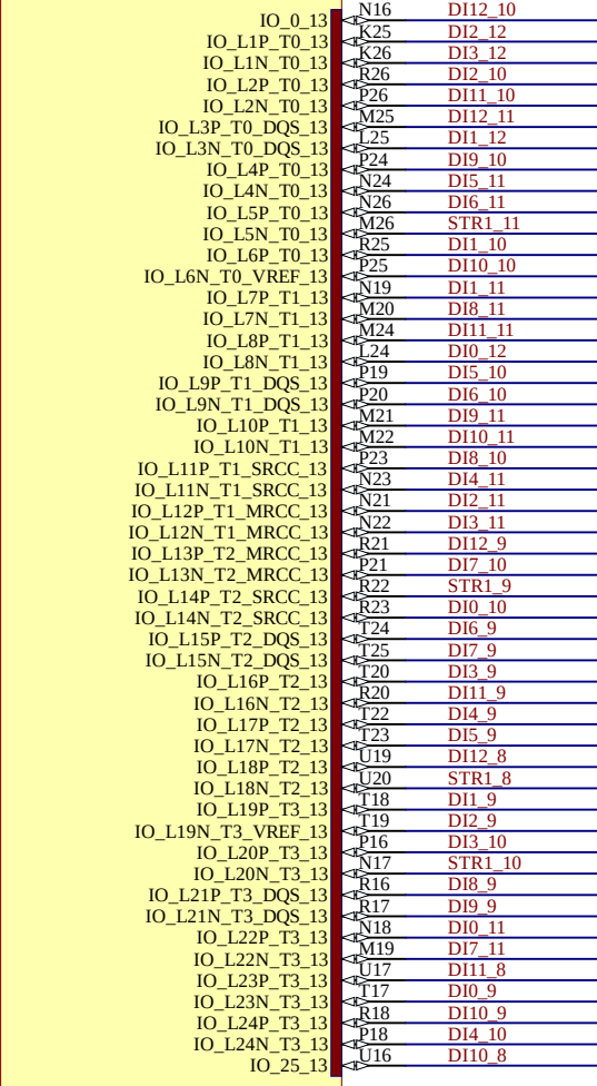
DD6B XC7K160T-2FBG676C
