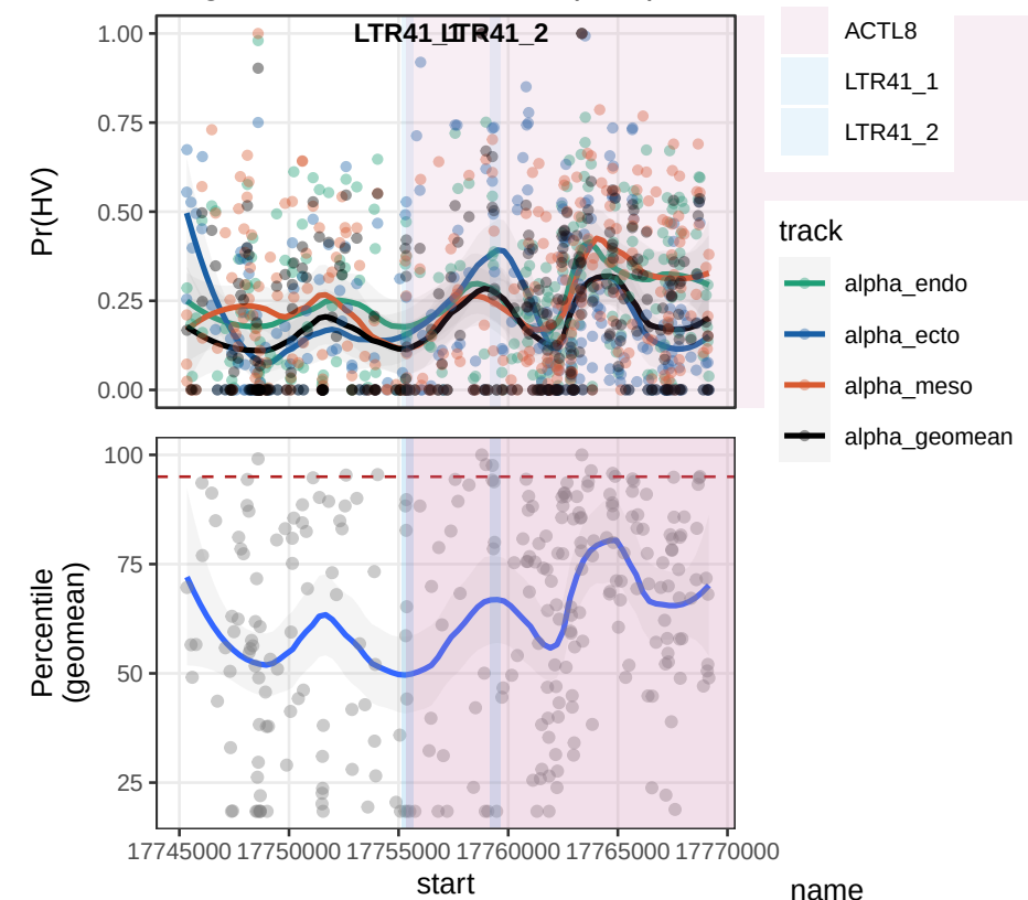
Region 2: ACTL8 / LTR41 (chr1) extended
