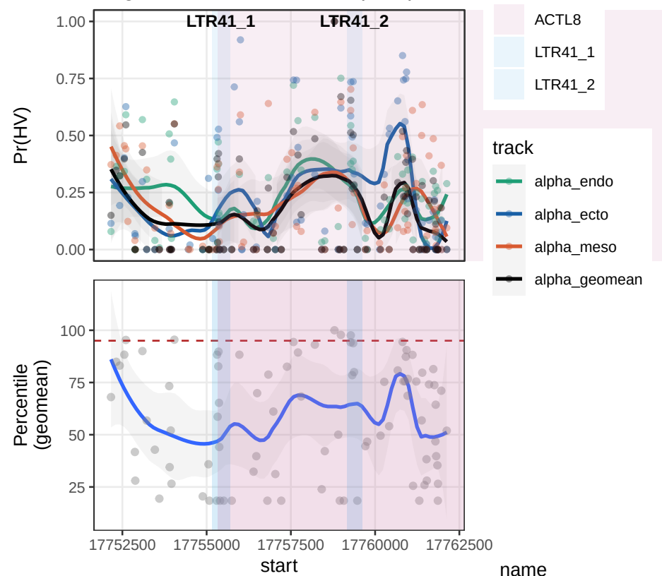
Region 2: ACTL8 / LTR41 (chr1)
