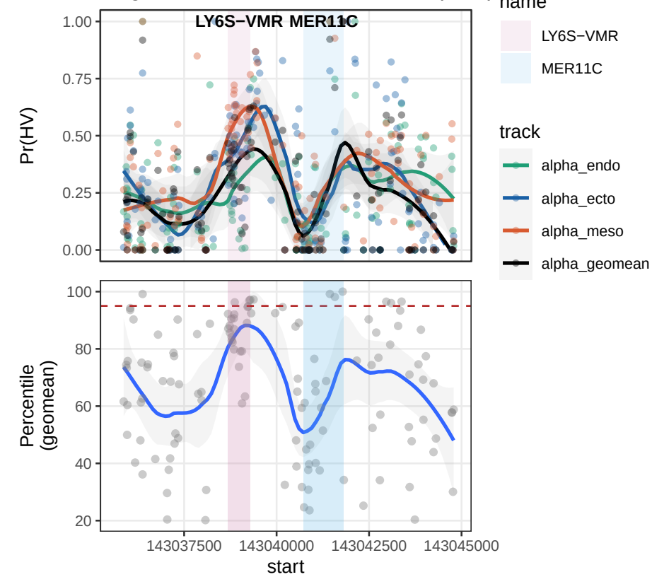
Region 1: LY6S-VMR / MER11C (chr8)
