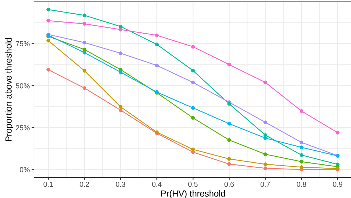
Based on one Pr(HV) per region
