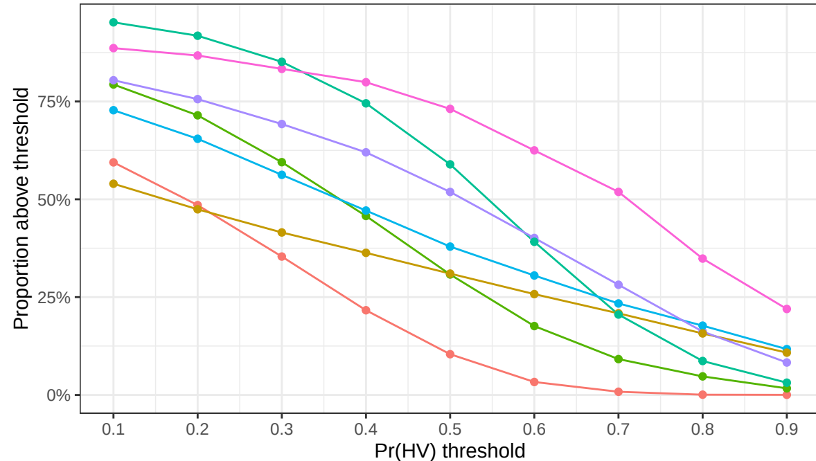
Based on one Pr(HV) per CpG
