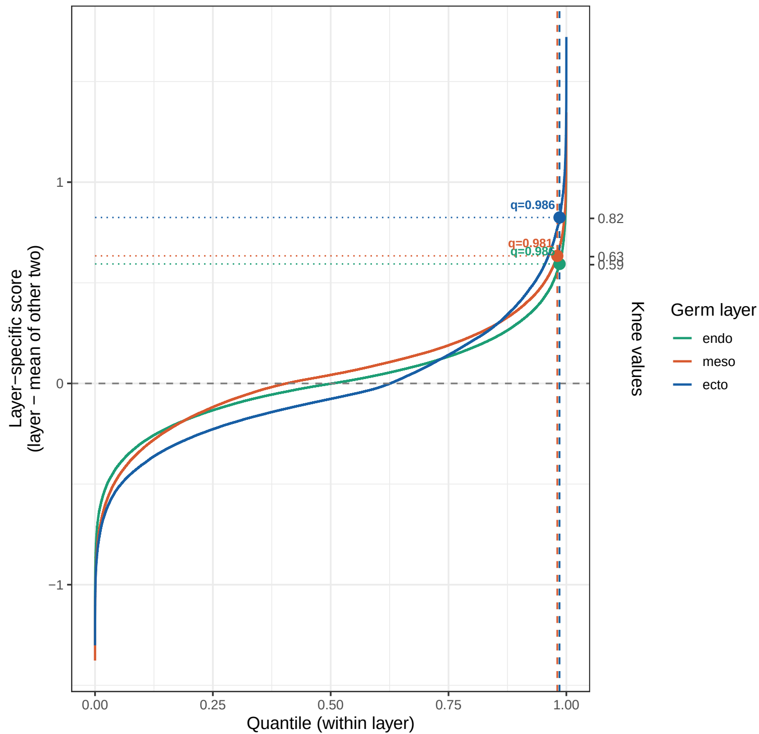
Per-CpG layer-specificity across the quantile distribution
