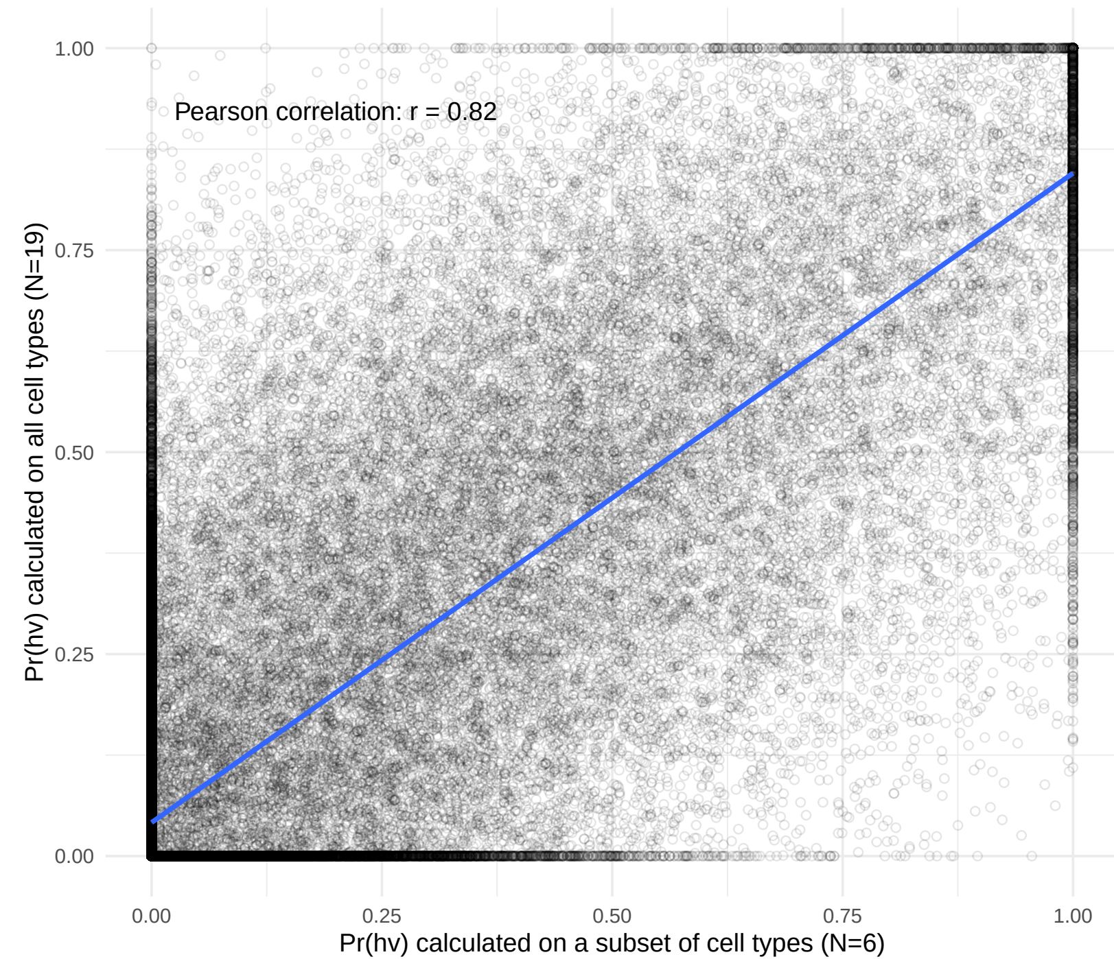
B Probability of being hypervariable in WGBS atlas mesoderm cell types (100k random CpG plotted)
