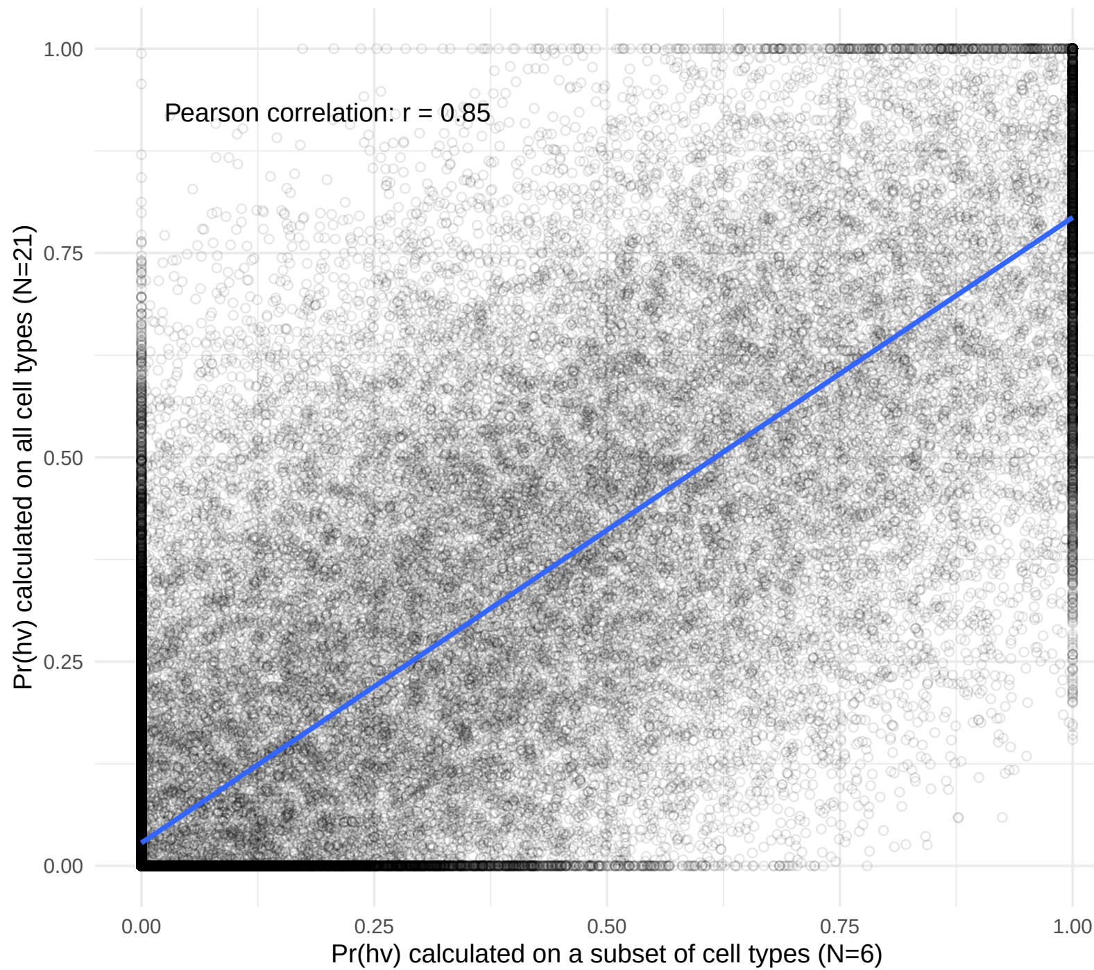
A Probability of being hypervariable in WGBS atlas endoderm cell types (100k random CpG plotted)
