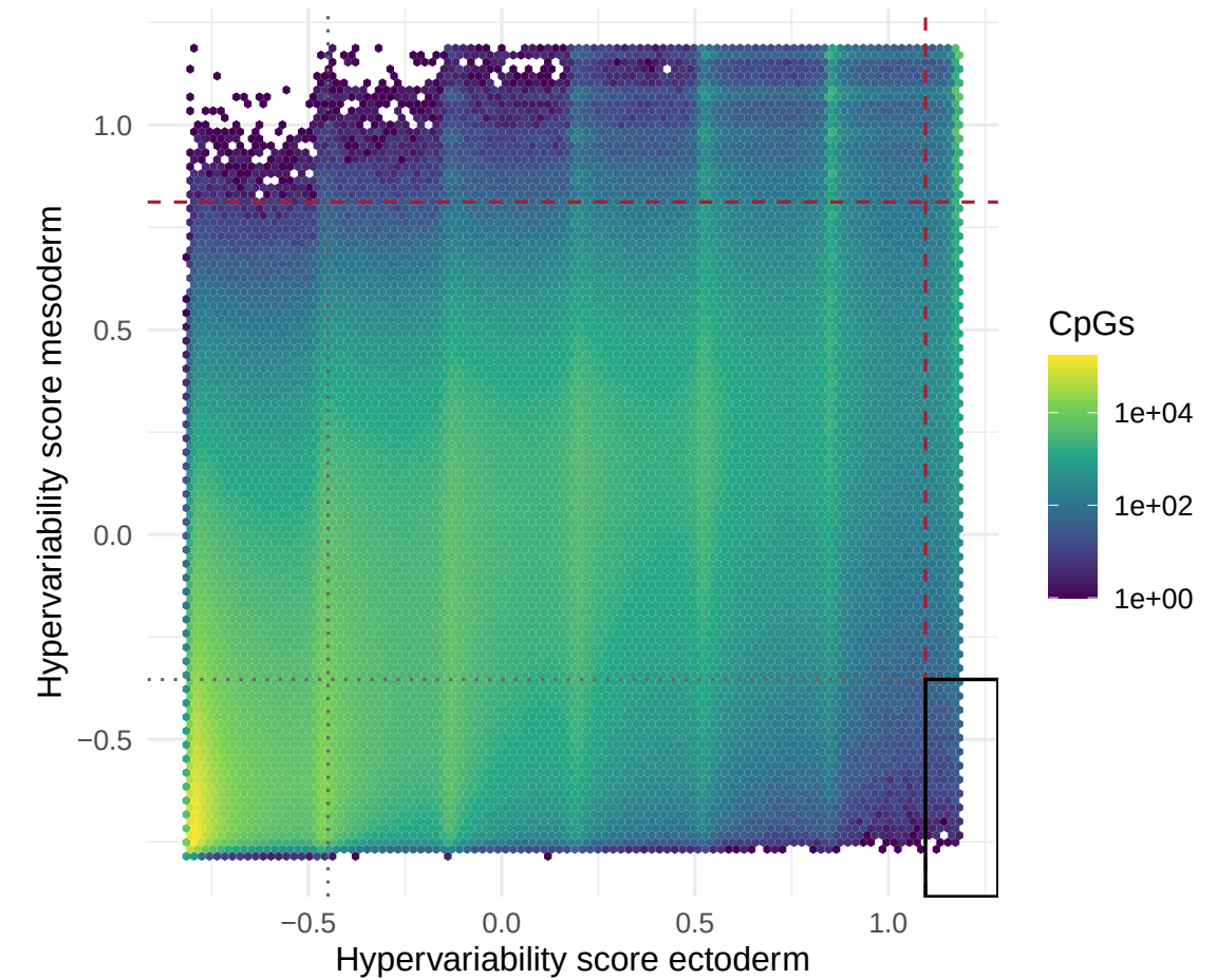
Hypervariability scores are strongly correlated
