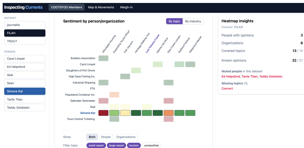
Figure 3.1: Heatmap
