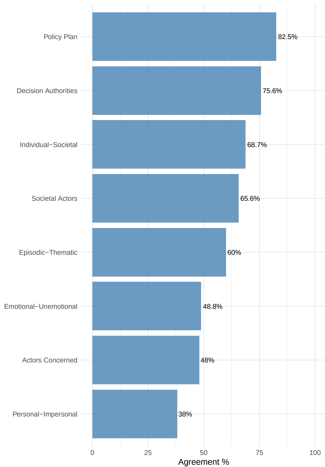
Inter-Coder Agreement (%)
