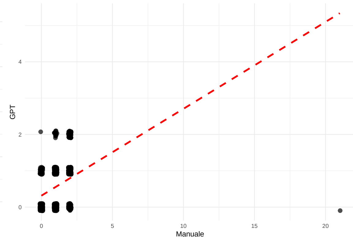
Inter-Coder: Emotional-Unemotional
