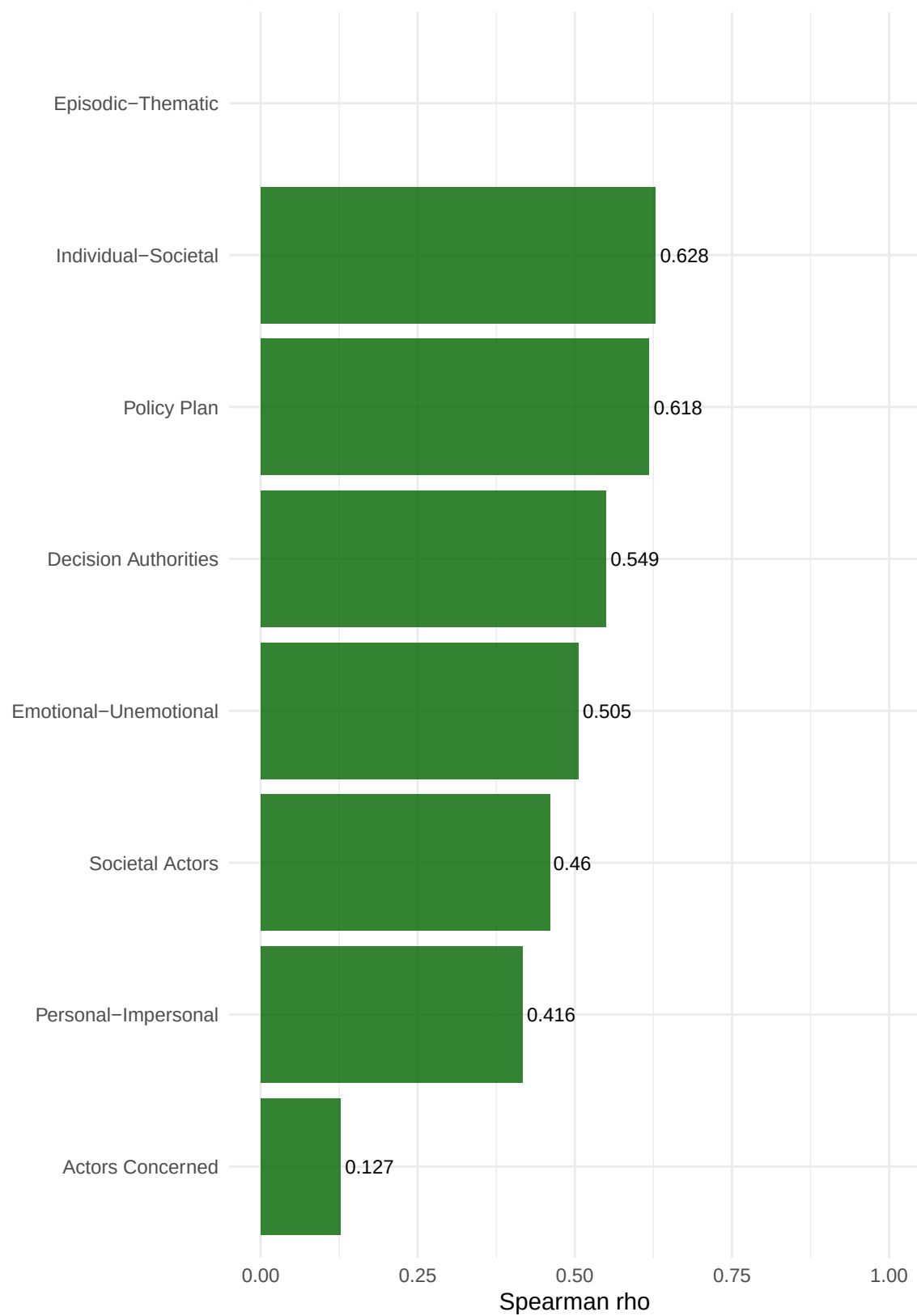
Spearman Correlation
