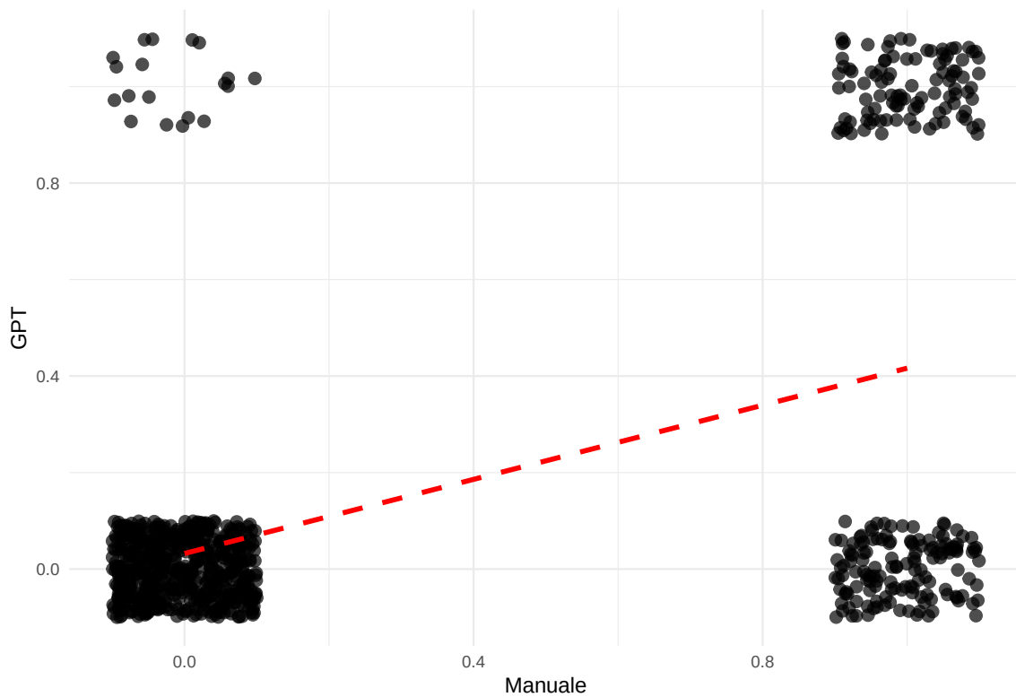
Inter-Coder: Policy Plan Agreement: 80.6% | Spearman: 0.497
