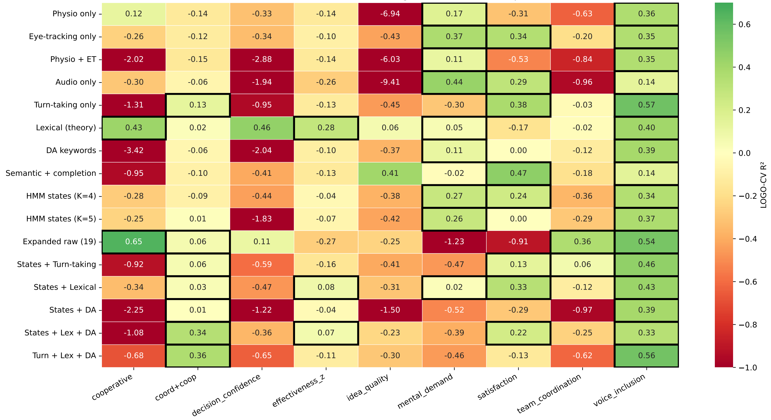
Feature-set ablation — LOGO-CV Ridge R 2 (black border = p < 0.05)
