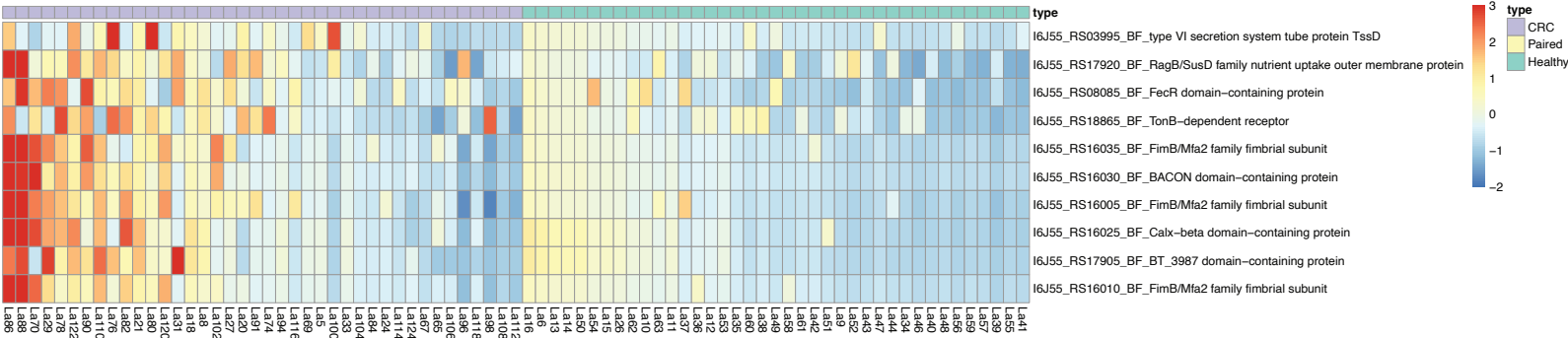
Figure 2. Z-score normalized expression of the top 10 upregulated B. fragilis genes across all samples in the CRC vs. Healthy comparison. Host-unmapped RNA-seq reads were processed using SAMSA2, then aligned with DIAMOND against the B. fragilis reference proteome (NCBI accession GCF_016889925.1). Differential expression was performed with DESeq2; genes were ranked by log2 fold change (CRC vs. Healthy) and the top 10 upregulated genes are shown. Healthy samples are mucosal colon biopsies from individuals with no observed gastrointestinal diseases. Columns represent
