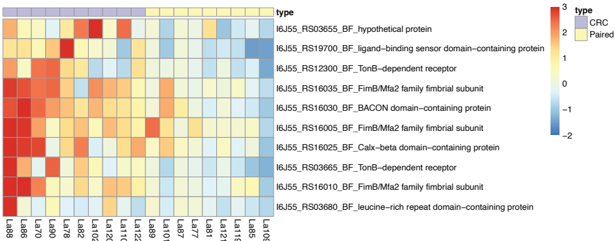
Figure 3 option 3. Filtered to an arbitrary subset of 10 patients.
