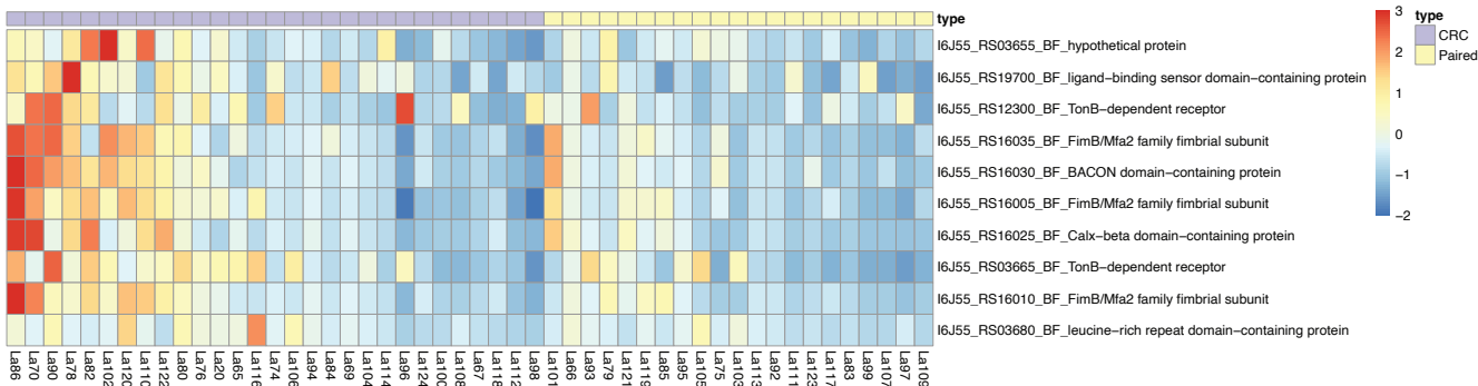
Figure 3 option 2. Filtered to samples with more than 100,000 total unmapped, ribodepleted reads.
