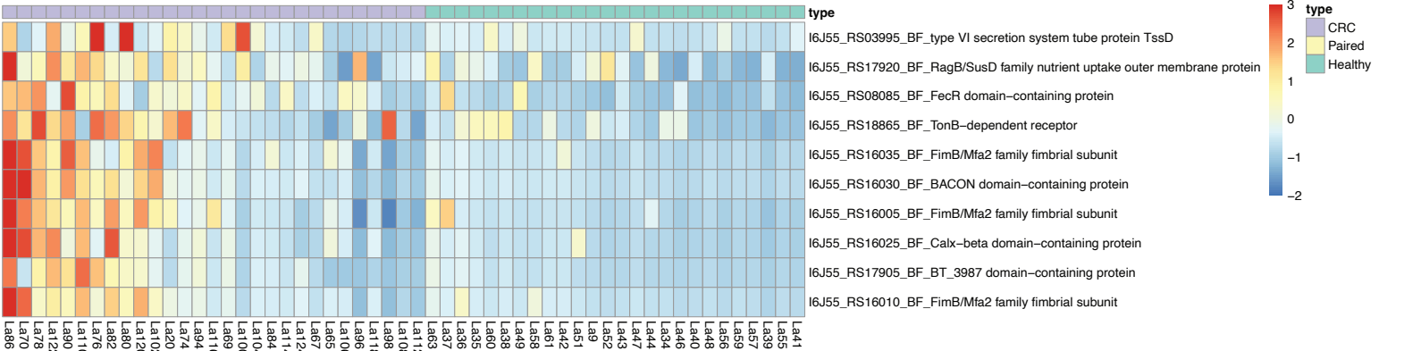
Figure 3 option 2. Filtered to samples with more than 100,000 total unmapped, ribodepleted reads.
