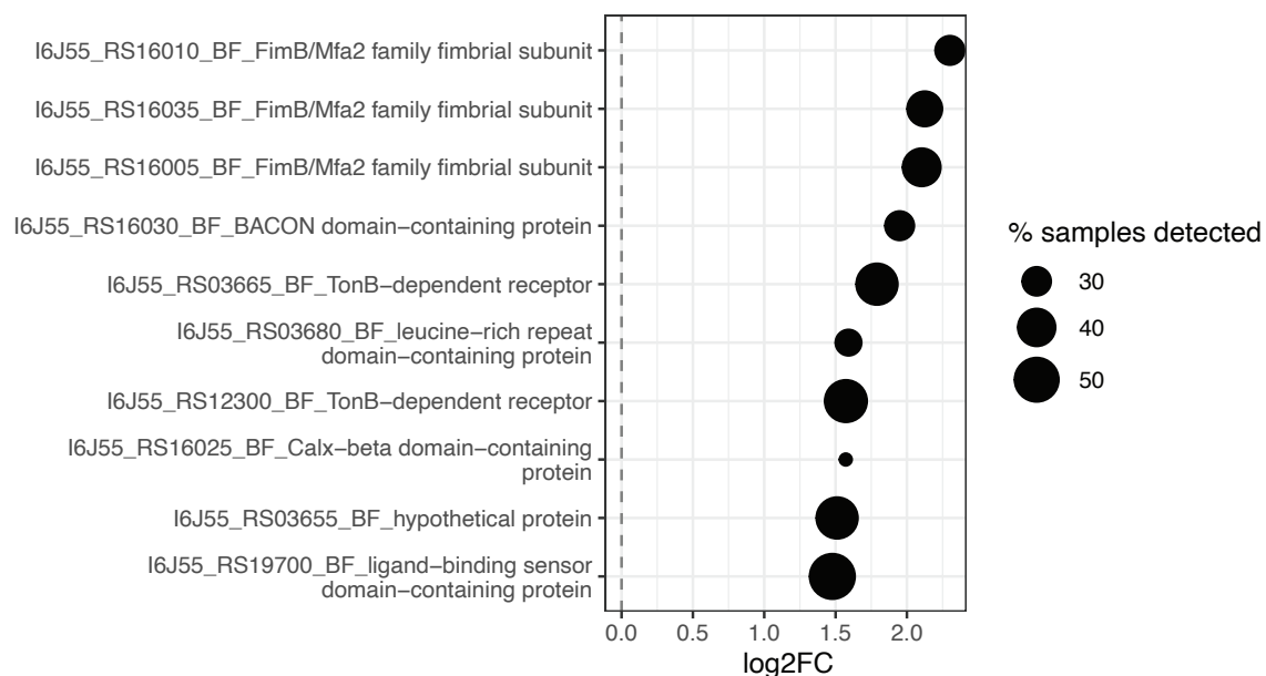
Figure 2. Log2 fold change of the top 10 upregulated B. fragilis genes between matched tumor and adjacent normal tissue (CRC vs. Paired) from DESeq2 analysis of host-unmapped RNA-seq reads aligned with DIAMOND against the B. fragilis reference proteome (GCF_016889925.1). Genes are ranked by \log_2FC , and point size indicates the percentage of samples in which each gene was detected.
