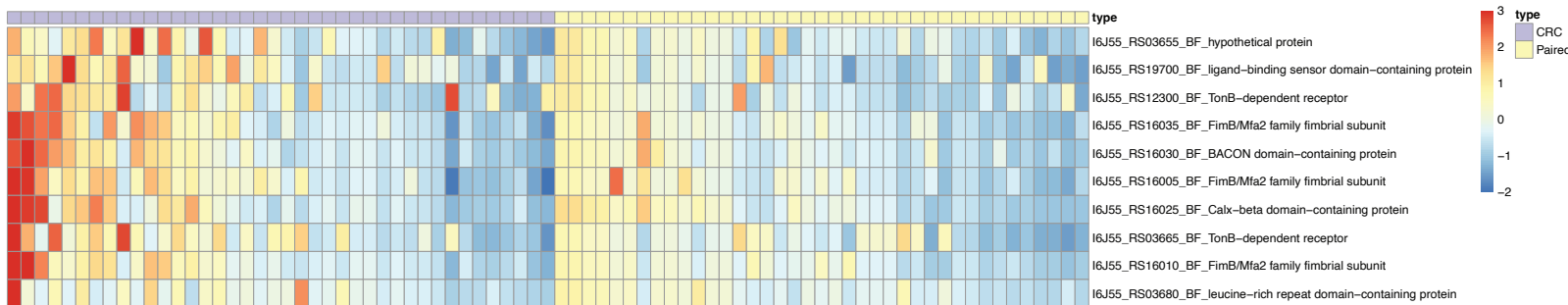
Figure 3. Z-score normalized expression of the top 10 upregulated B. fragilis genes across all samples in the CRC vs. Paired comparison. Host-unmapped RNA-seq reads were processed using SAMSA2, then aligned with DIAMOND against the B. fragilis reference proteome (NCBI accession GCF_016889925.1). Differential expression was performed with DESeq2; genes were ranked by log2 fold change (CRC vs. Paired) and the top 10 upregulated genes are shown. Columns represent individual samples grouped by tissue type (CRC or Paired) and sorted by descending total z-score within each group. Color reflects row-wise z-score.
