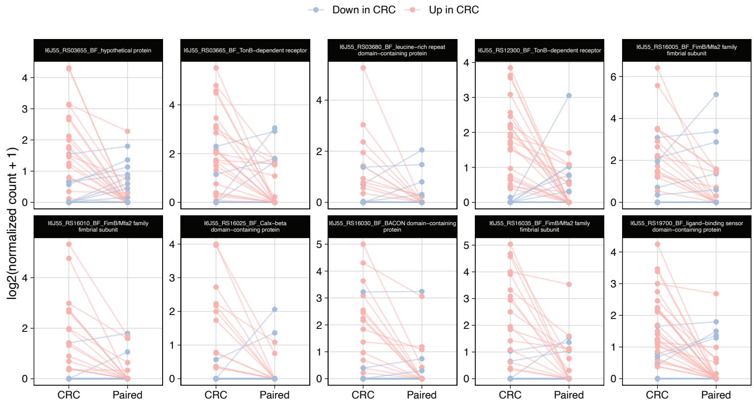
Figure 1. Per-patient expression of the top 10 differentially expressed B. fragilis genes between matched tumor and adjacent normal tissue. Mucosal colon biopsies were collected from CRC patients (any T-stage) at Zealand University Hospital. Paired samples consist of a tumor biopsy (CRC) and a biopsy from normal mucosa >10 cm from the tumor (Paired) from the same patient. Host-unmapped RNA-seq reads were processed using SAMSA2, aligned with DIAMOND against the B. fragilis reference proteome (NCBI accession GCF_016889925.1). Differential expression was performed with DESeq2, genes were ranked by \log_2FC (CRC vs. Paired), and the top 10 upregulated genes are shown. Each line connects a single patient's tumor-associated CRC and non-tumor associated paired sample. Point colour indicates the direction of change for that patient (red = higher in CRC, blue = lower in CRC). Y-axis shows \log_2(\text{DESeq2 size-factor normalized count} + 1) .
