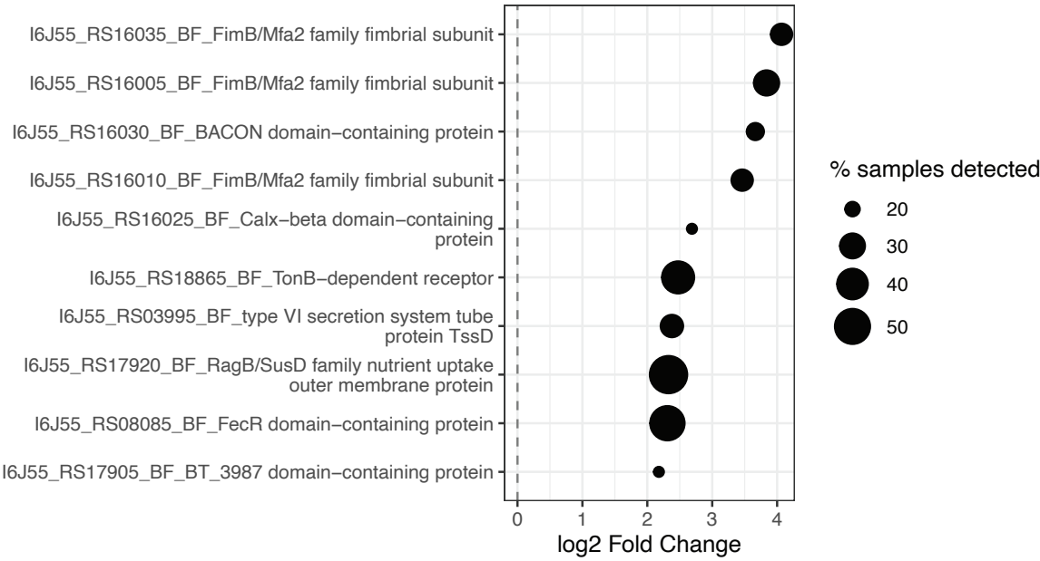
Figure 1. Log2FC of the top 10 upregulated B. fragilis genes between tumor tissue from CRC patients and mucosal colon biopsies from healthy individuals with no observed gastrointestinal diseases (CRC vs. Healthy), from DESeq2 analysis of host-unmapped RNA-seq reads aligned with DIAMOND against the B. fragilis reference proteome (GCF_016889925.1). Genes are ranked by log2 fold change and point size indicates the percentage of samples in which each gene was detected.
