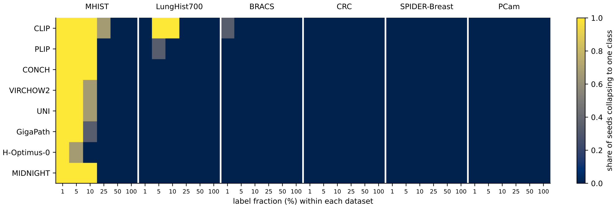
Single-class collapse of the linear probe
