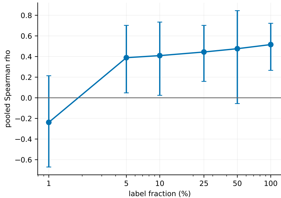
Pooled over 48 cells cluster bootstrap over datasets, 95% CI
