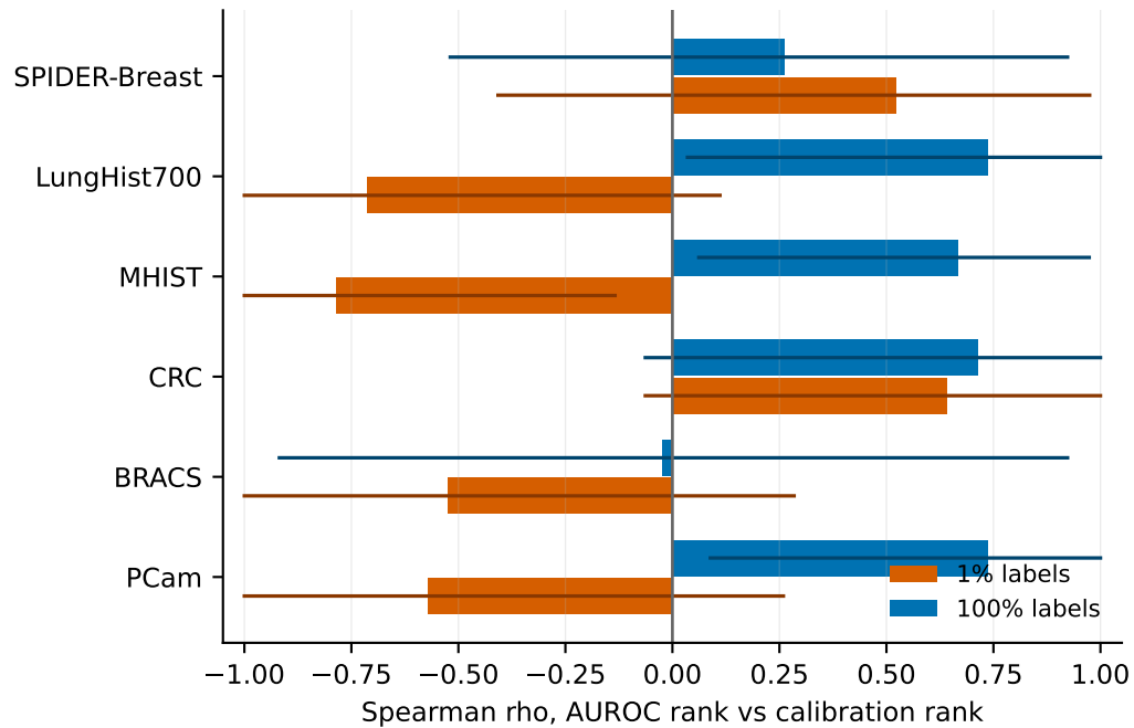
Per dataset, with bootstrap intervals
