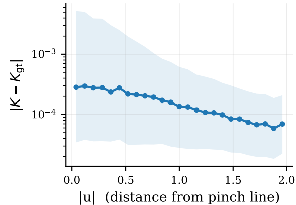
Gaussian curvature K
