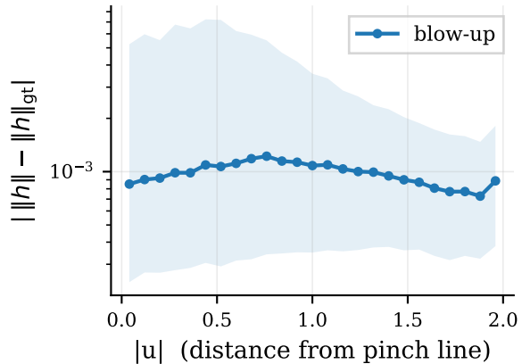
Total curvature \|h\|
