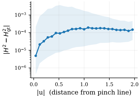
Squared mean curvature H^2
