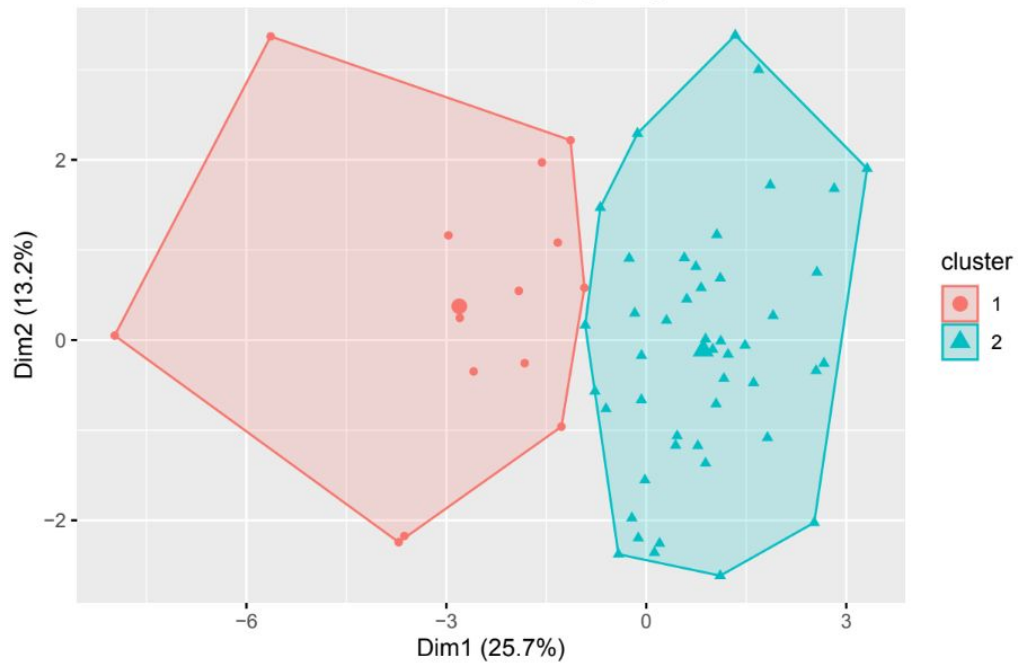
Student Clusters Based on Sustainability Responses
