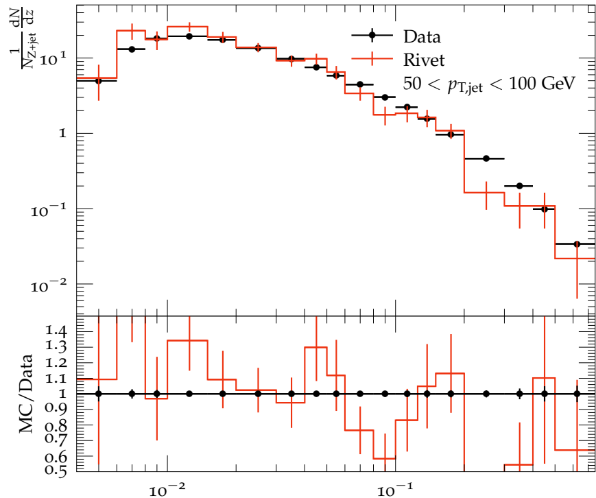
Distributions of the longitudinal momentum fraction of the hadron
