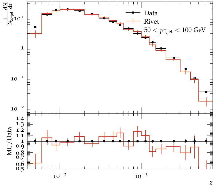
Distributions of the longitudinal momentum fraction of the hadron
