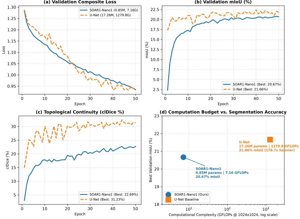
Figure 4: Empirical convergence dynamics and computational Pareto frontier comparing SOAR1-Nano1 (0.85M params) against U-Net (17.26M params) on MAGFiLO (1024 × 1024). (Top-left) Monotonic composite loss progression; (Top-right) Validation mIoU trajectories; (Bottom-left) Centerline Dice (cIDice) connectivity; (Bottom-right) FLOPs vs. mIoU Pareto frontier on log scale, establishing SOAR’s 178.7× computational efficiency advantage.
