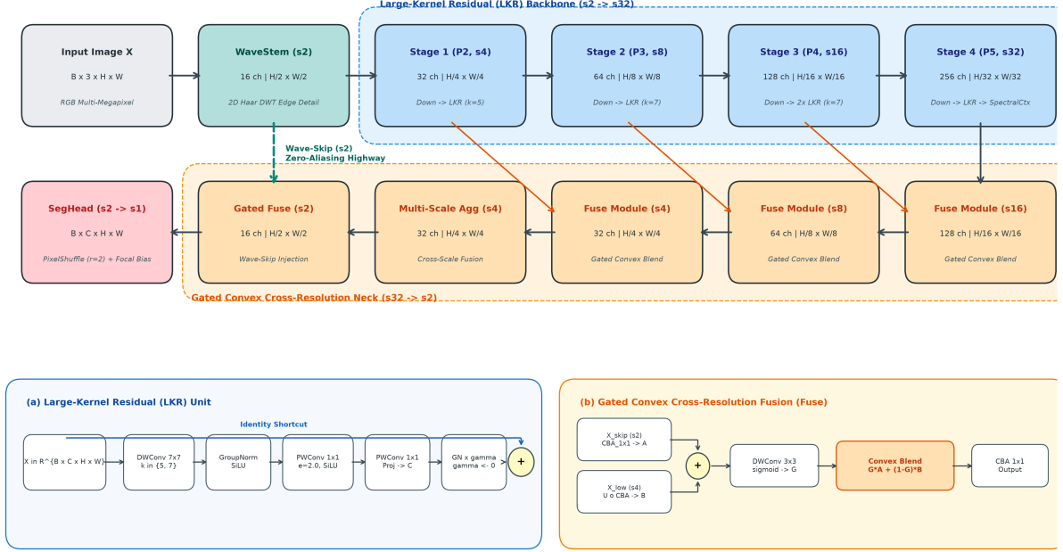
Figure 1: Comprehensive Architectural Framework of the SOAR Baseline. Sub-pixel high-frequency spatial gradients are captured at native stride s_2 by the zero-aliasing Wavelet Stem ( WaveStem ) and routed through a dedicated detail highway. Coarse contextual semantics are aggregated down to stride s_{32} via Large-Kernel Residual (LKR) depthwise blocks with zero-initialized Group Normalization ( \gamma \leftarrow 0 ), augmented by global spectral context ( SpectralCtx ). The top-down Gated Convex Cross-Resolution Fusion ( Fuse ) neck dynamically interpolates spatial detail and semantic abstraction via continuous combination fields G(u, v) \in [0, 1] . Sub-pixel periodic shuffling ( SegHead ) directly synthesizes full-resolution logits ( s_2 \rightarrow s_1 ) without bilinear interpolation blur.
