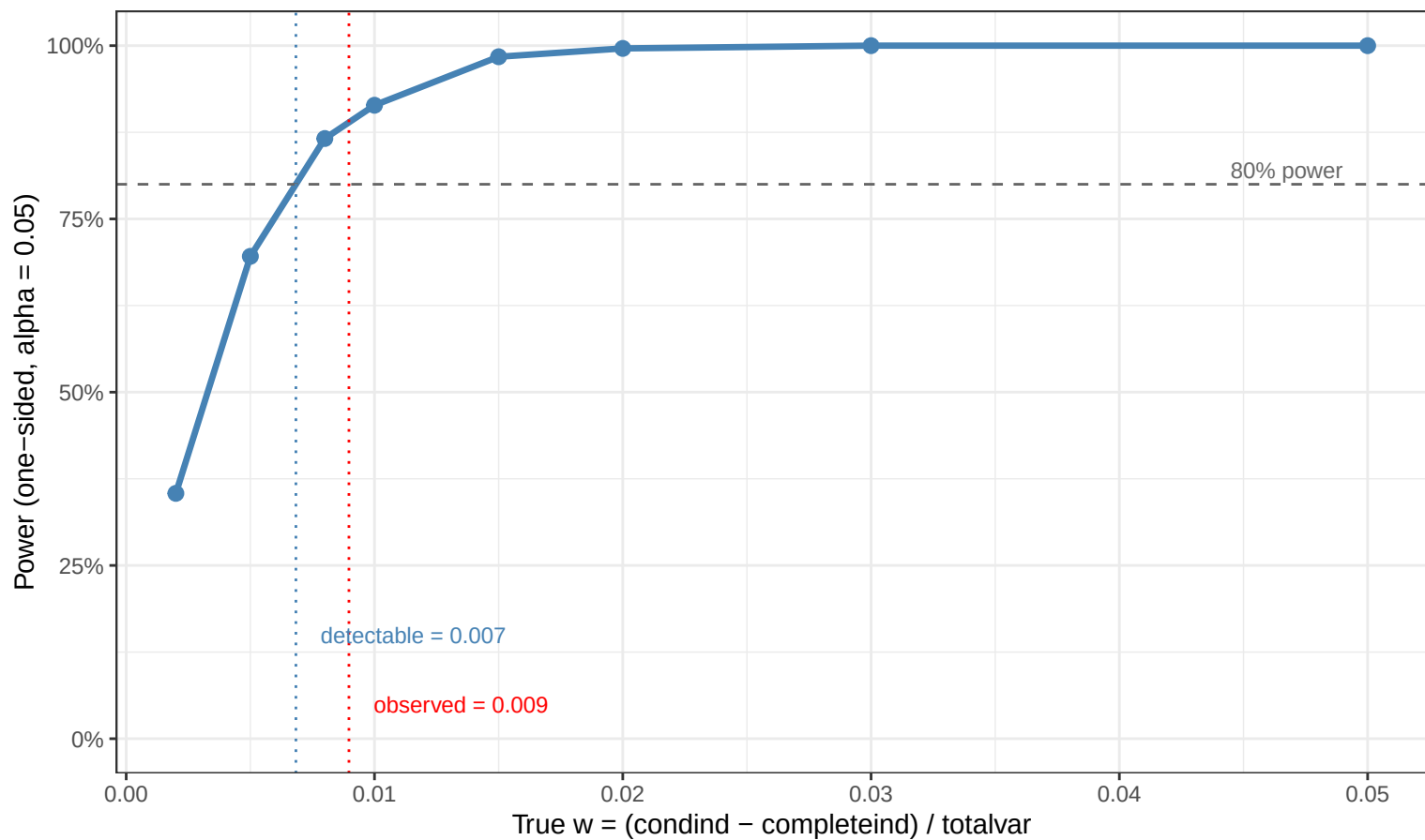
Power to detect within-family ascribed contribution – Sisters (N families=612)
