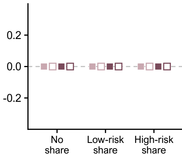
Belief update (intimacy)
