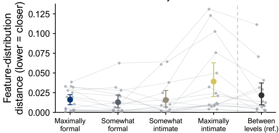
Study 3a
