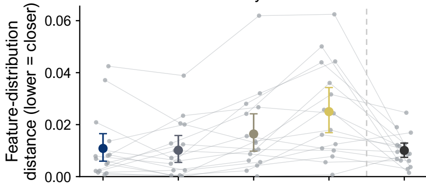
Study 3a
