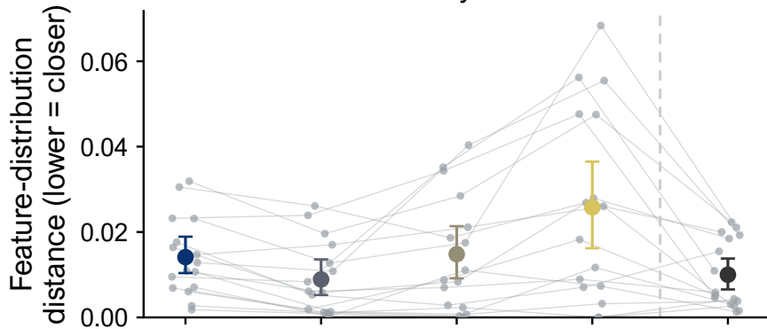
Study 1b
