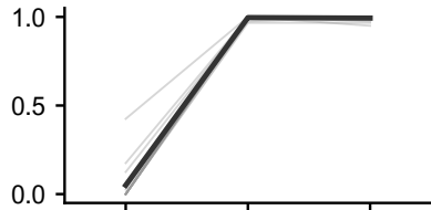
Goal-satisfaction g
