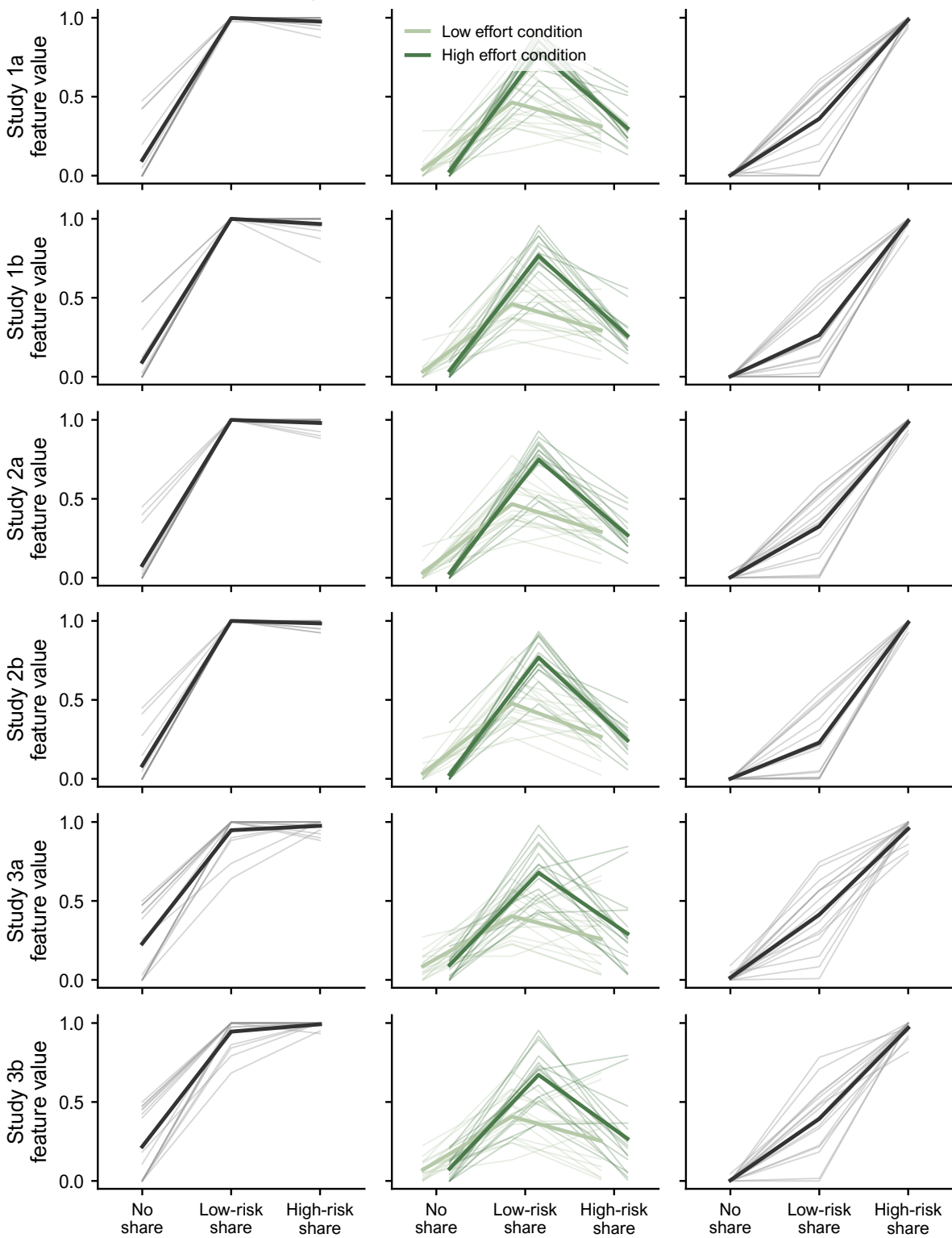
Goal-satisfaction g
