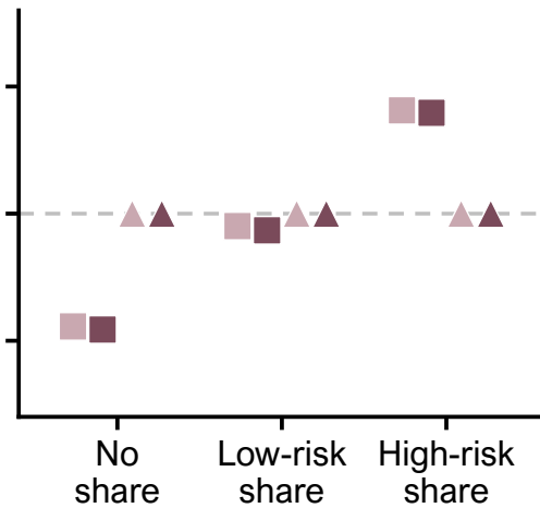
Discomfort-only
