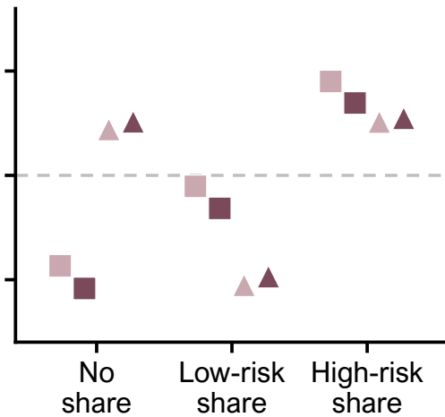
Full
