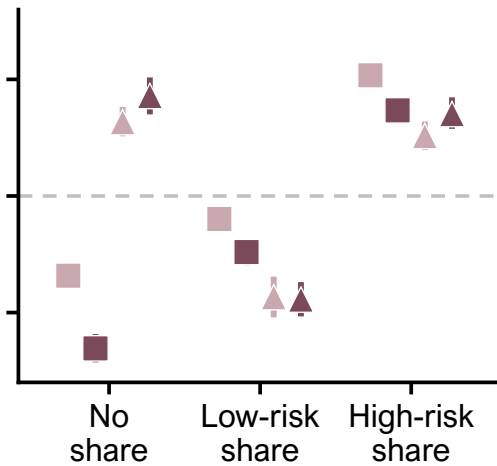
Humans
