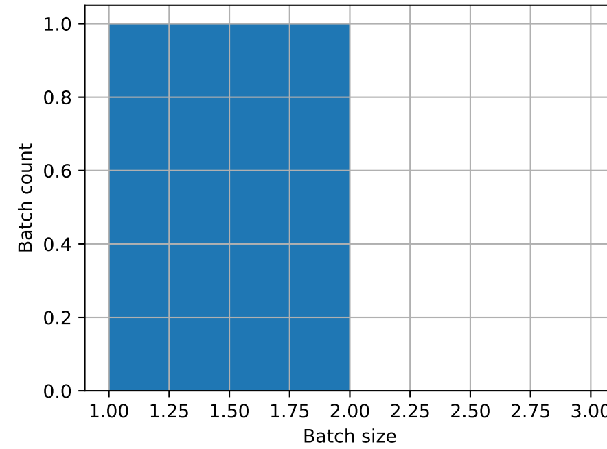
Model 15
