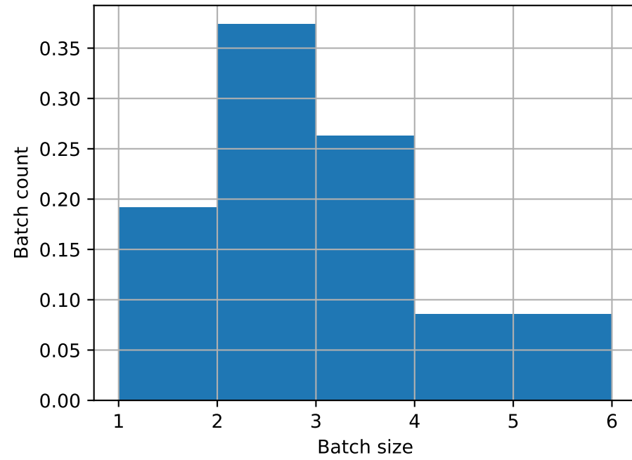
Model 14
