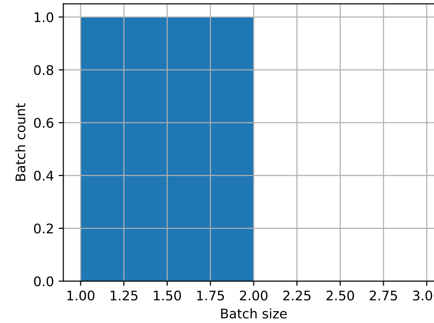
Model 16
